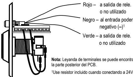
Figure 9 – Vista lateral
