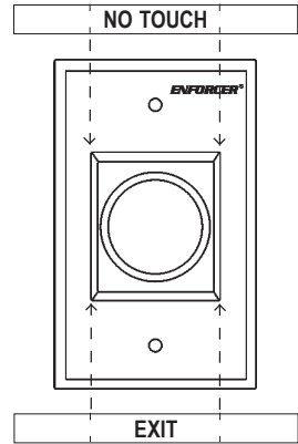
Fig. 2 – Decal Alignment
