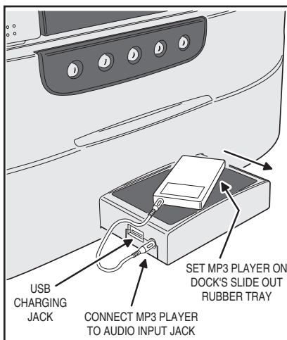
Figure 19. MP3 Player on Device Drawer
