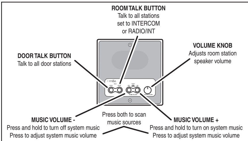
Figure 15. 4-Wire Room Station and Patio Station Intercom Controls
