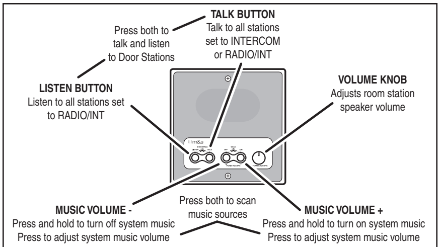
Figure 14. 4-Wire Room Station and Patio Station Intercom Controls
