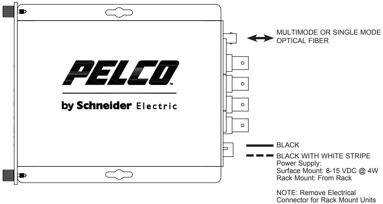
FIGURE 1 – FTV/FRV80D2(M,S)1(ST,FC) TRANSMITTER AND RECEIVER
