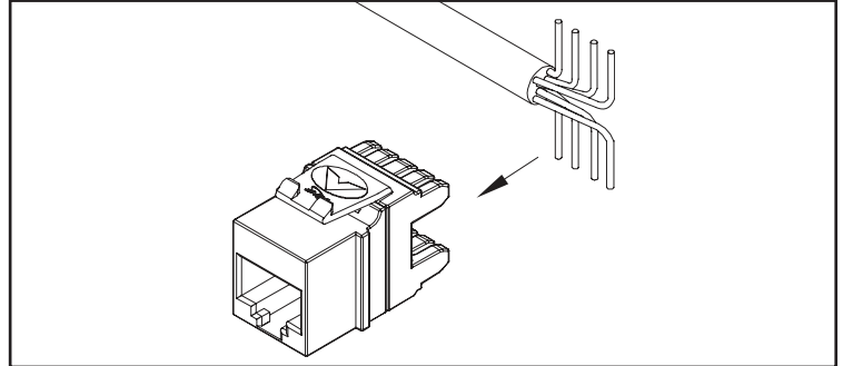
Step 1. Determine wiring scheme T568A or T568B.
