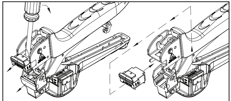
Step 2. Use a flat-head screwdriver to remove the EZ blade and seat. Then replace with the HD blade.
