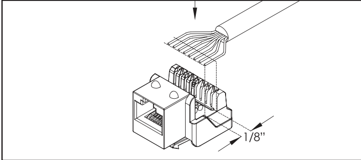
Step 1. Determine wiring scheme T568A or T568B.
