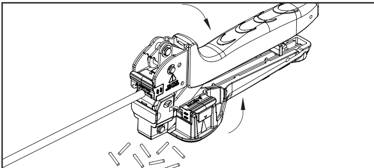
Step 3. Squeeze the handle and terminate.
