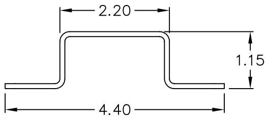
CEILING SUPPORT BRACKET
