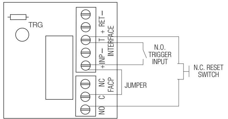
Fig. 10 Normally Open FACP Latching trigger input with reset: (This output has not been evaluated by UL)
