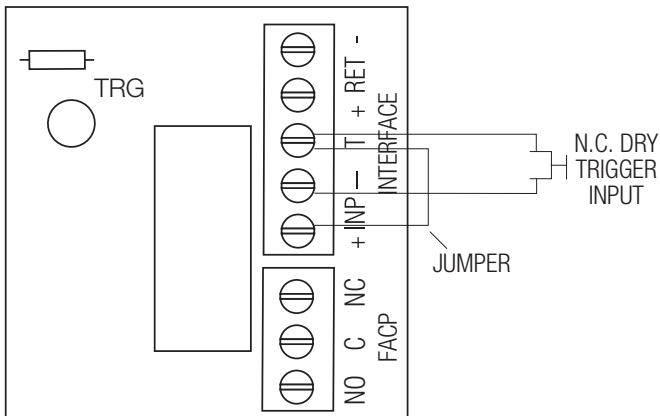
Fig. 11 Normally Closed - Non-Latching FACP trigger input:
