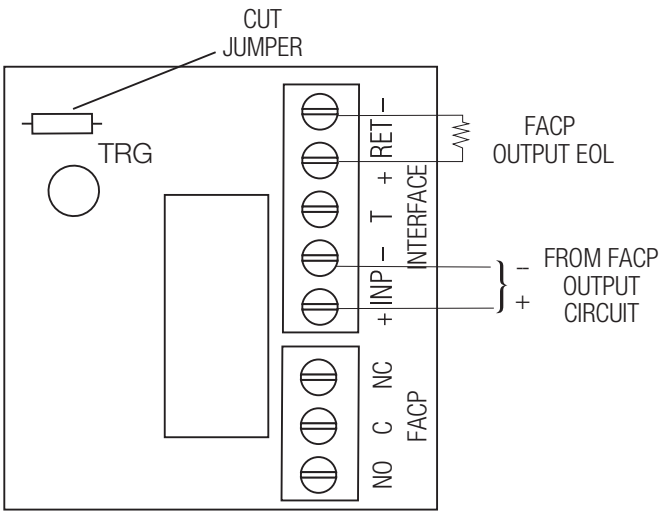
Fig. 9 Normally Open - Non-Latching FACP trigger input:
