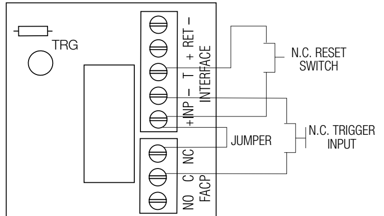
Fig. 9 Normally Closed - Latching FACP trigger input with reset: (This output has not been evaluated by UL)
