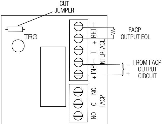
Fig. 6 Normally Open - Non-Latching FACP trigger input:
