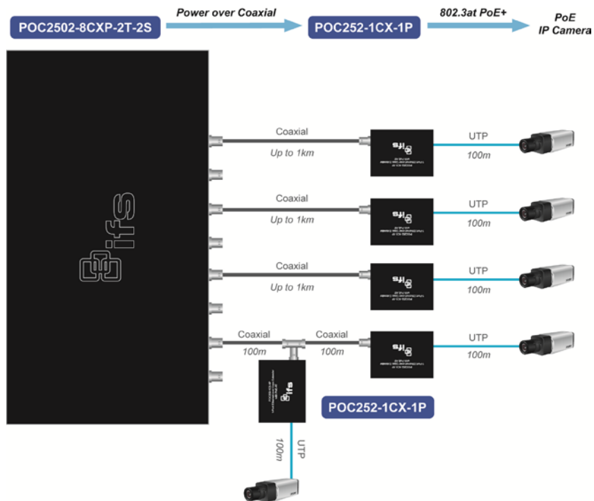
Typical POC to IP Camera Configuration
