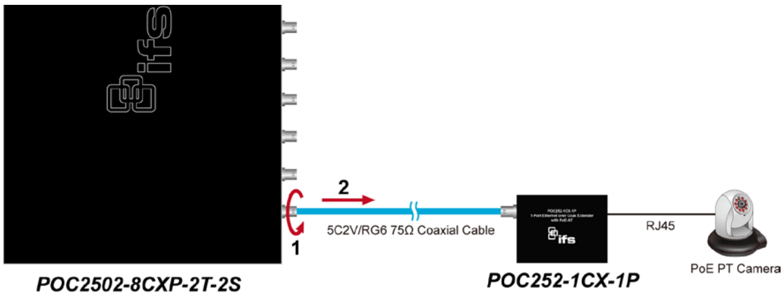
Figure 2-1-8 How to pull out the coaxial cable from POC Managed Switch
