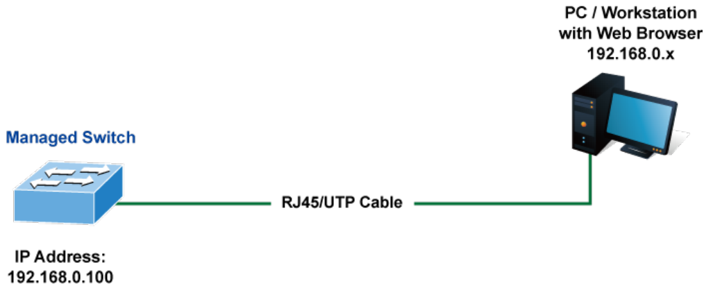
Figure 3-1-3 Web Management
