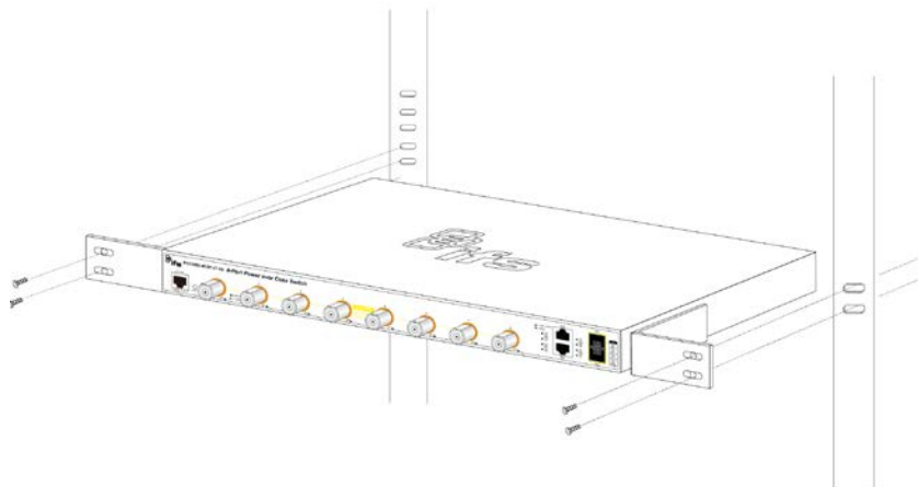
Figure 2-1-6 Mounting POC Managed Switch in a Rack
