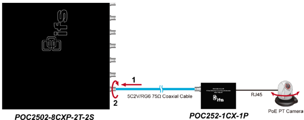
Figure 2-1-8 How to insert the coaxial cable from POC Managed Switch
