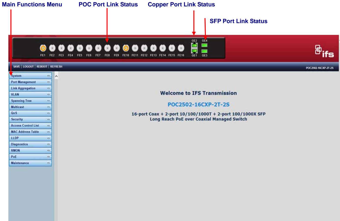
Figure 4-1-4 Main Page
