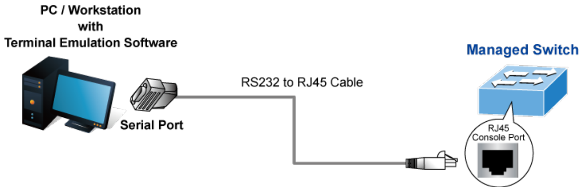
Figure 3-1-1: Console Management
