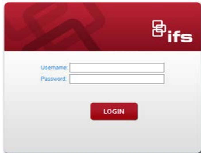
Figure 4-1-2 Login screen
