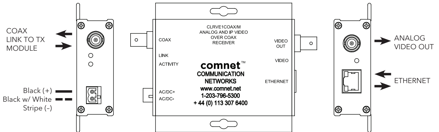
FIGURE 2 - CLRVE1COAX/M RECEIVER
