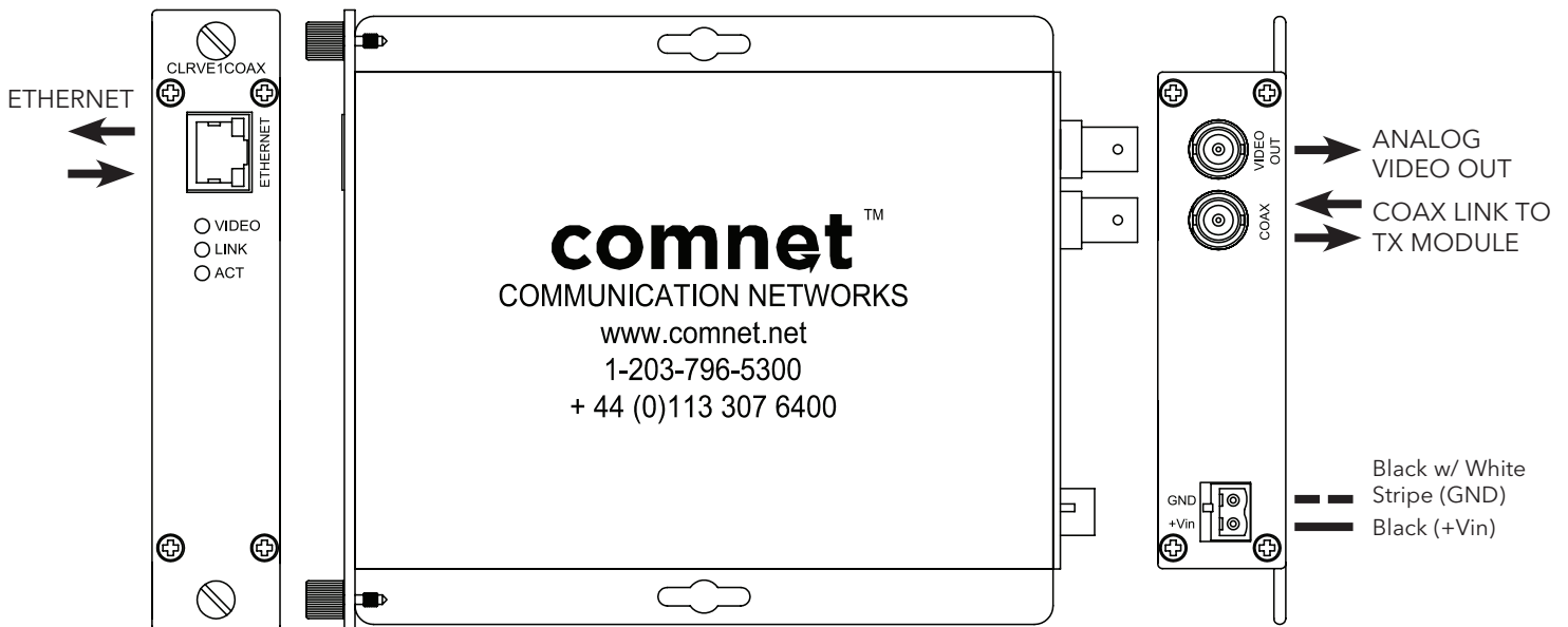
FIGURE 4 - CLRVE1COAX RECEIVER
