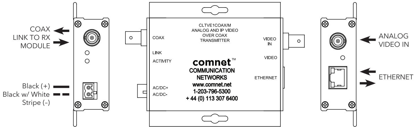
FIGURE 1 - CLTVE1COAX/M TRANSMITTER
