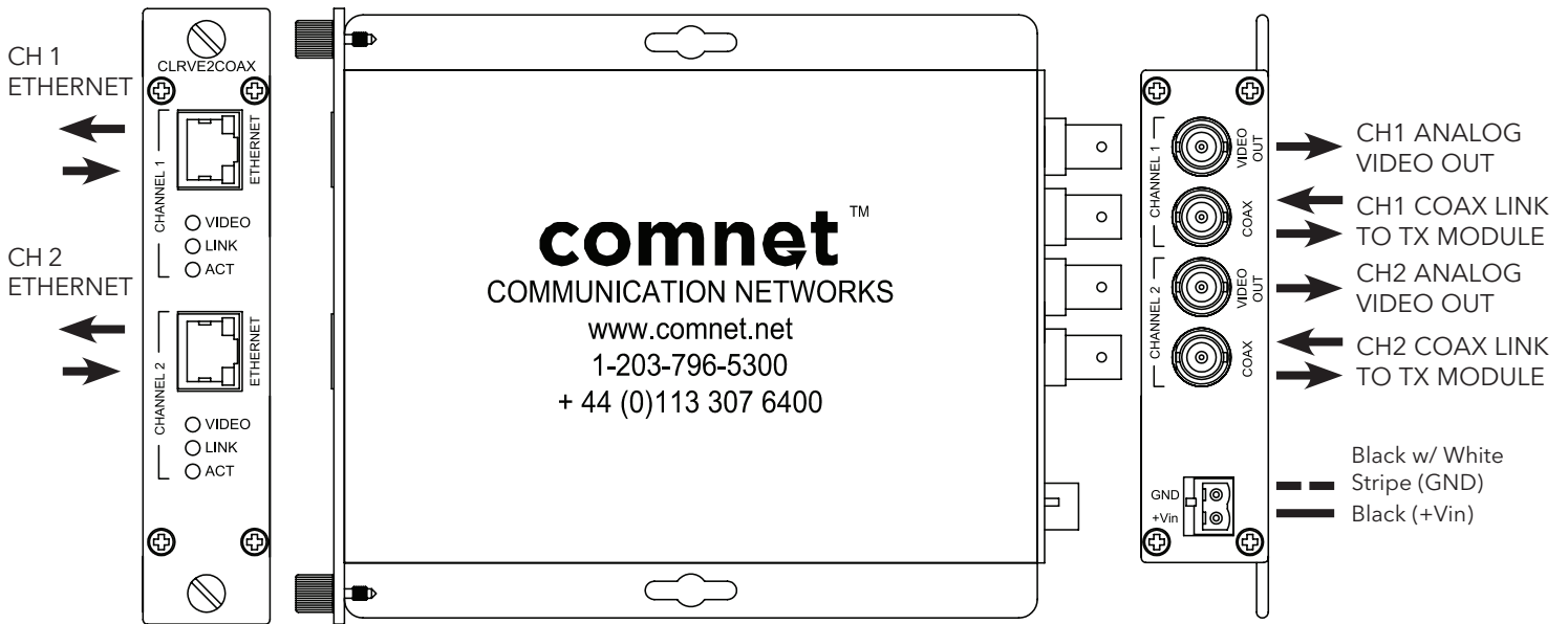
FIGURE 5 - CLRVE2COAX RECEIVER
