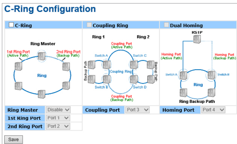
C-Ring interface
