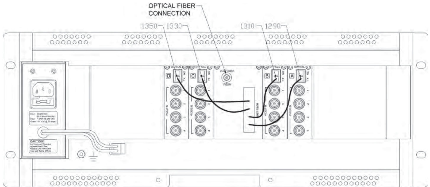
FIGURE 3 – FVT160M1 TRANSMITTER FRONT AND REAR
