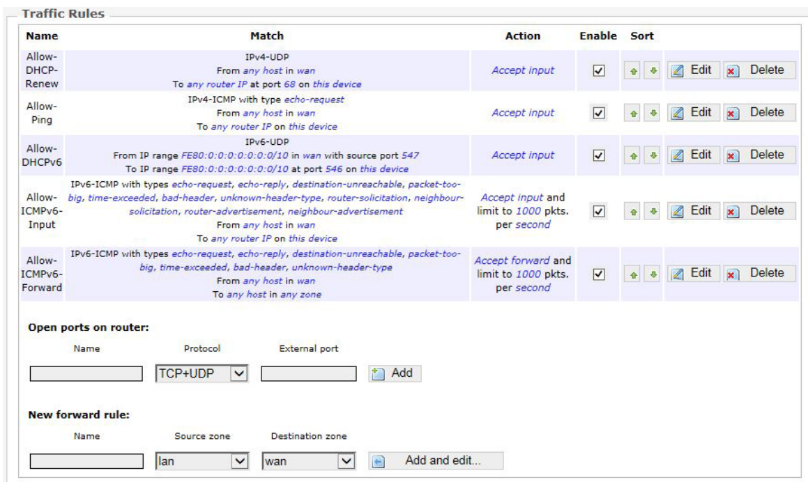
Figure 52: Firewall Traffic Rules with the default settings.
