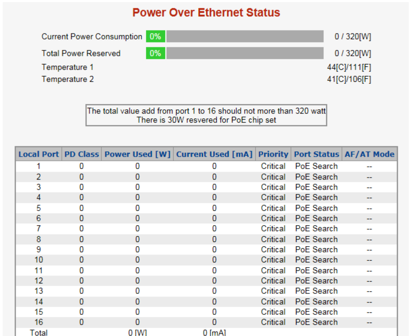
Figure 4-16-1: Power over Ethernet Status
