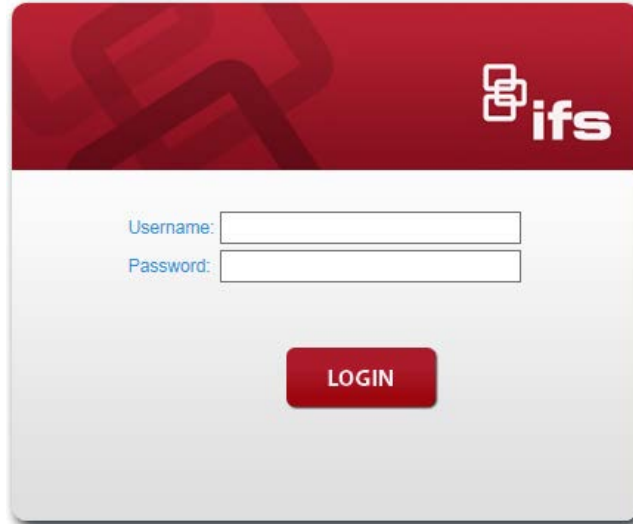
Figure 4-1-2: Login Screen
