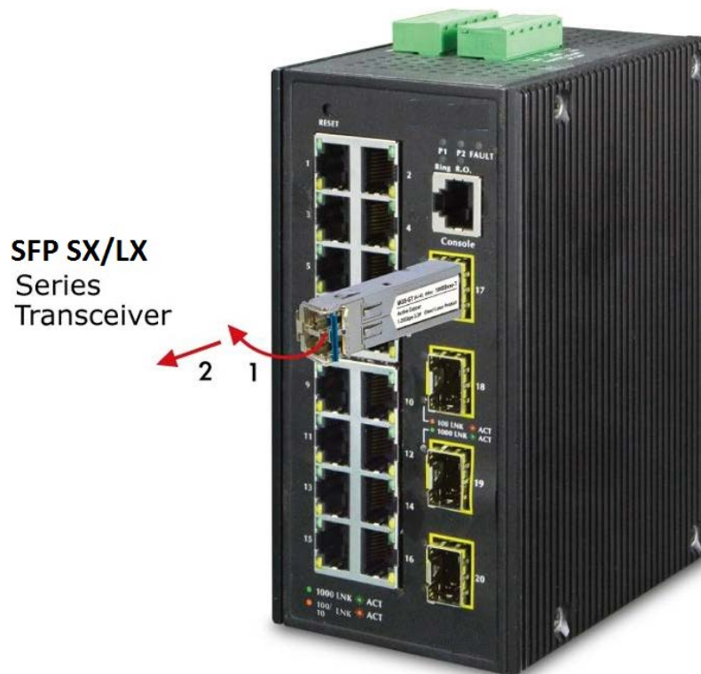
Figure 2-26: Pull out the SFP Transceiver Module
