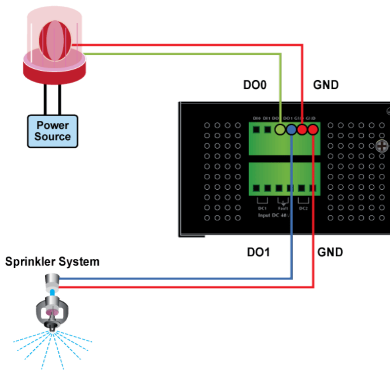
Figure 2-24 Wires DO0 and DO1 to Open Detector
