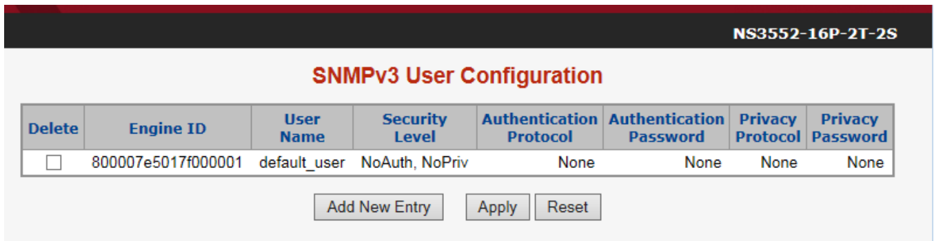
Figure 4-3-5: SNMPv3 Users Configuration page Screenshot
