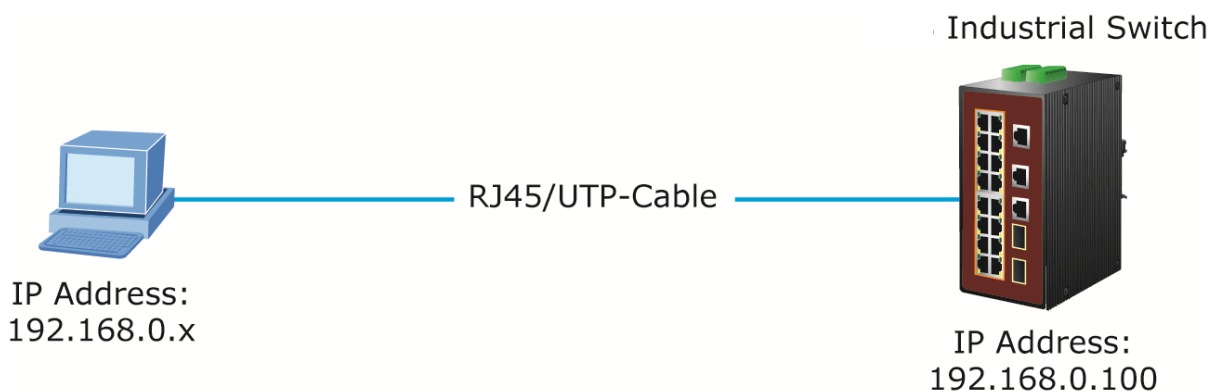
Figure 4-1-1: Web Management
