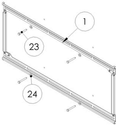
Step 3: Mounting the wall plate
