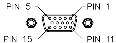
REAR VIEW
