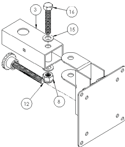
Step 4: Attaching the swivel bracket to the support tube.
