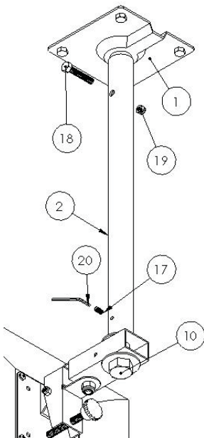
Step 7: Connecting the extension tube to the ceiling plate
