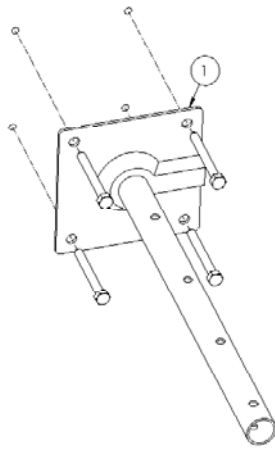
Step 3: Attaching the ceiling plate to the ceiling. (Lag Screws not included)
