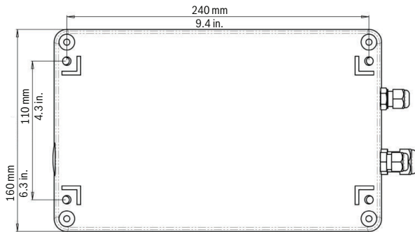
Power Supply Box – bottom view
