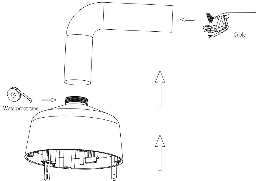
FIGURE 2-7: INDOOR / OUTDOOR PENDANT CABLING
