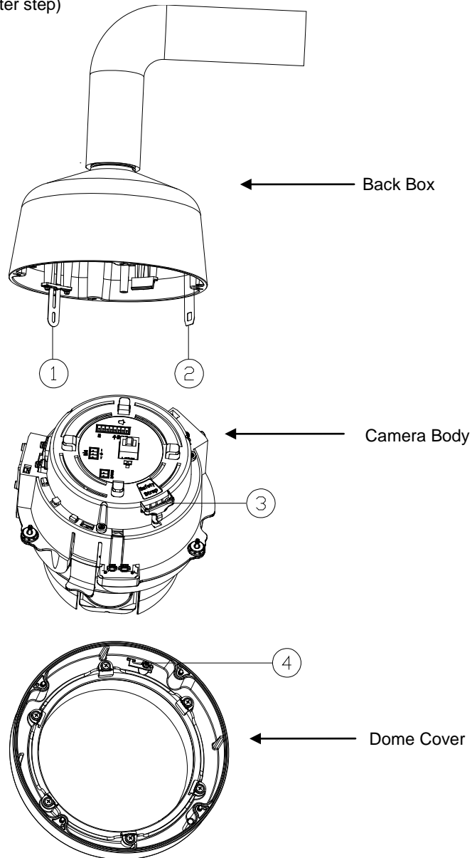
FIGURE 2-8: INDOOR / OUTDOOR PENDANT ALIGNING
