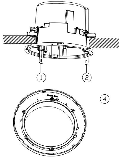
FIGURE 2-15: Attaching the Lower Dome
