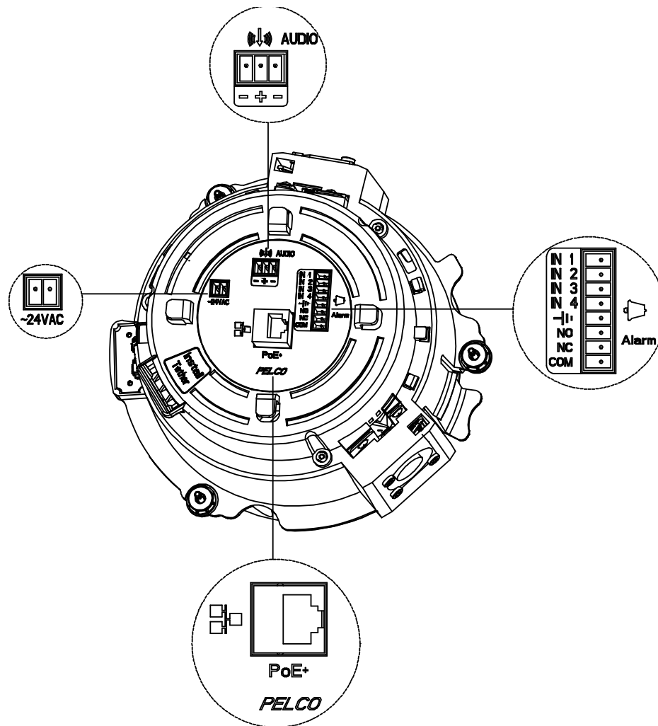
FIGURE 2-2: CONNECTORS FOR WIRING
