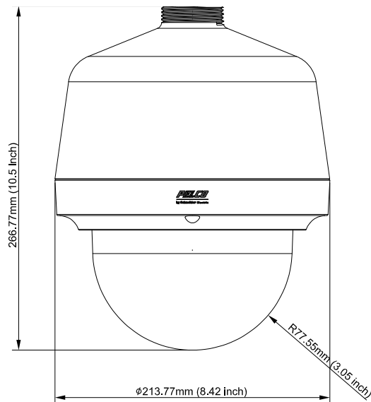
PTZ Dome Outdoor/Indoor Pendant Mount
