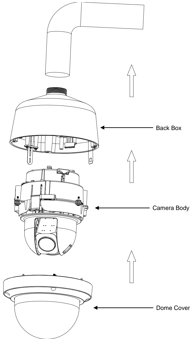
FIGURE 2-9: INDOOR / OUTDOOR PENDANT INSTALLATION
