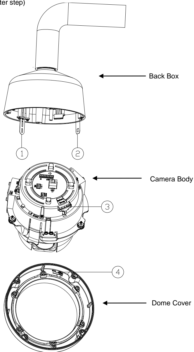
FIGURE 2-4: INDOOR / OUTDOOR PENDANT ALIGNING
