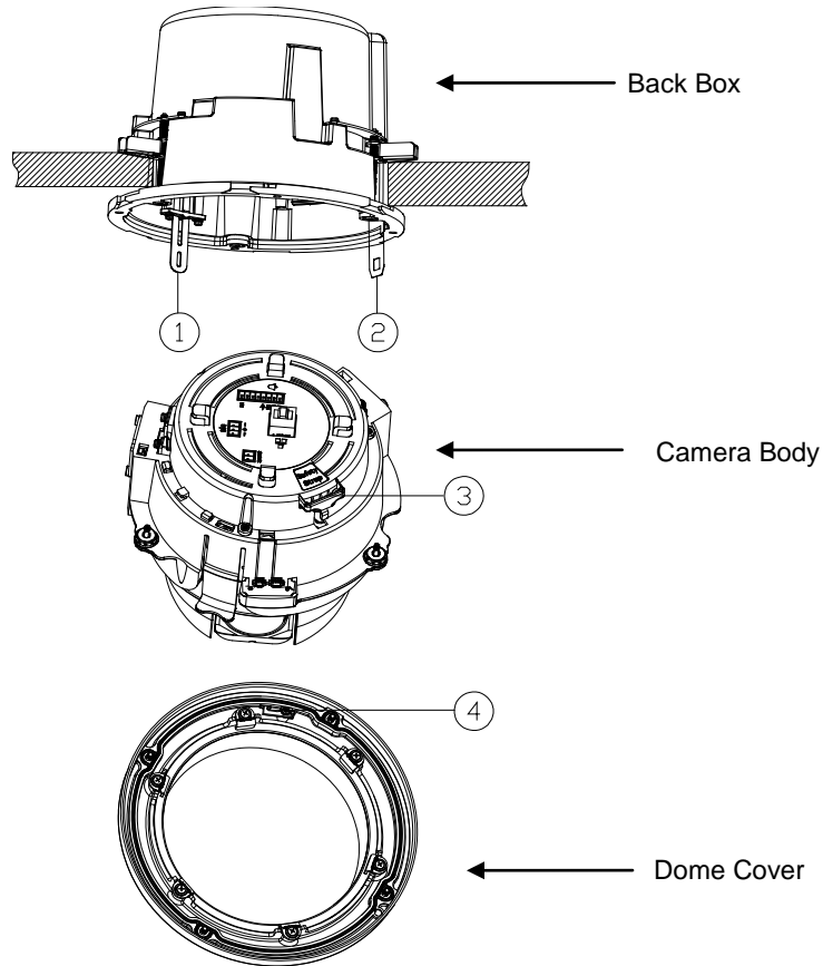
FIGURE 2-14: OUTDOOR IN-CEILING ALIGNING
