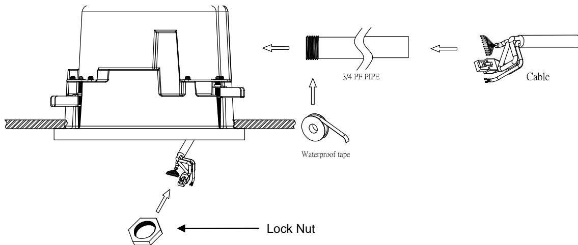
FIGURE 2-13: OUTDOOR IN-CEILING CABLING
