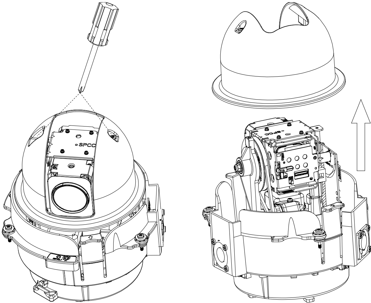
FIGURE 2-1: DISASSEMBLE THE CAMERA
