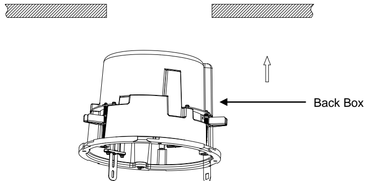
FIGURE 2-11: INSERTING THE BACK BOX
