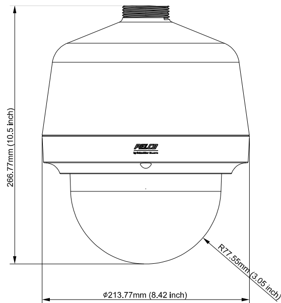
PTZ Dome Outdoor/Indoor Pendant Mount
