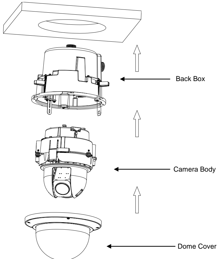
FIGURE 2-16: OUTDOOR IN-CEILING INSTALLATION
