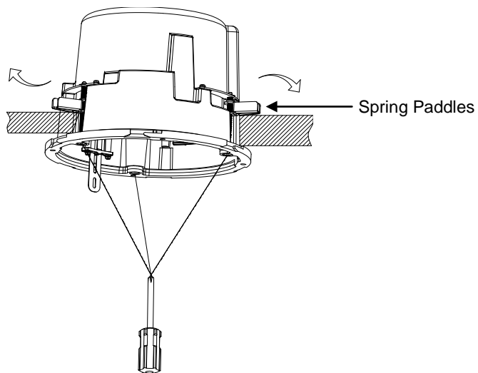
FIGURE 2-12: SECURING THE BACK BOX
