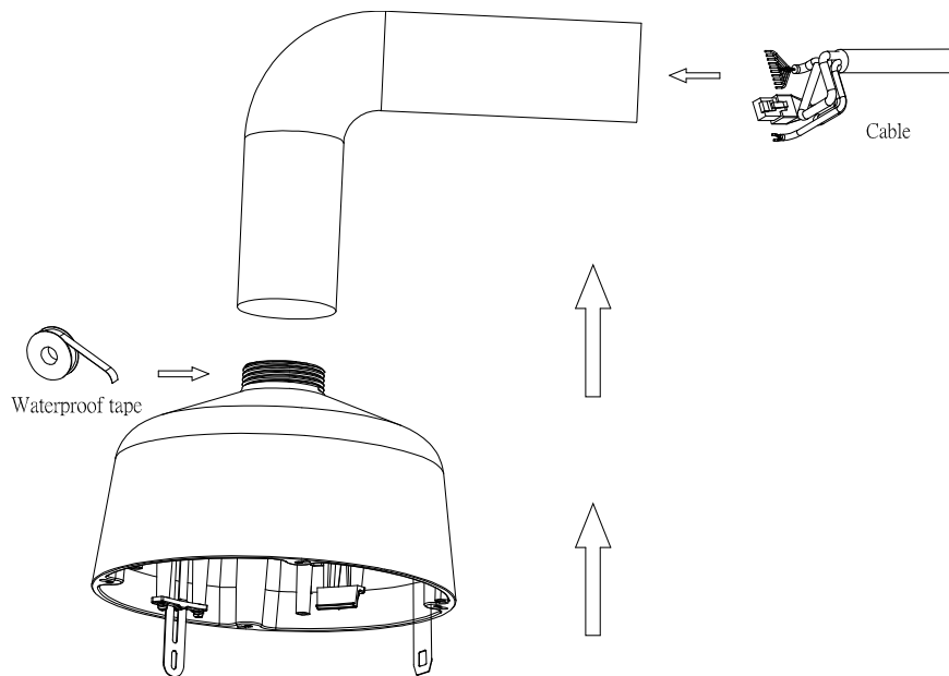
FIGURE 2-3: INDOOR / OUTDOOR PENDANT CABLING
