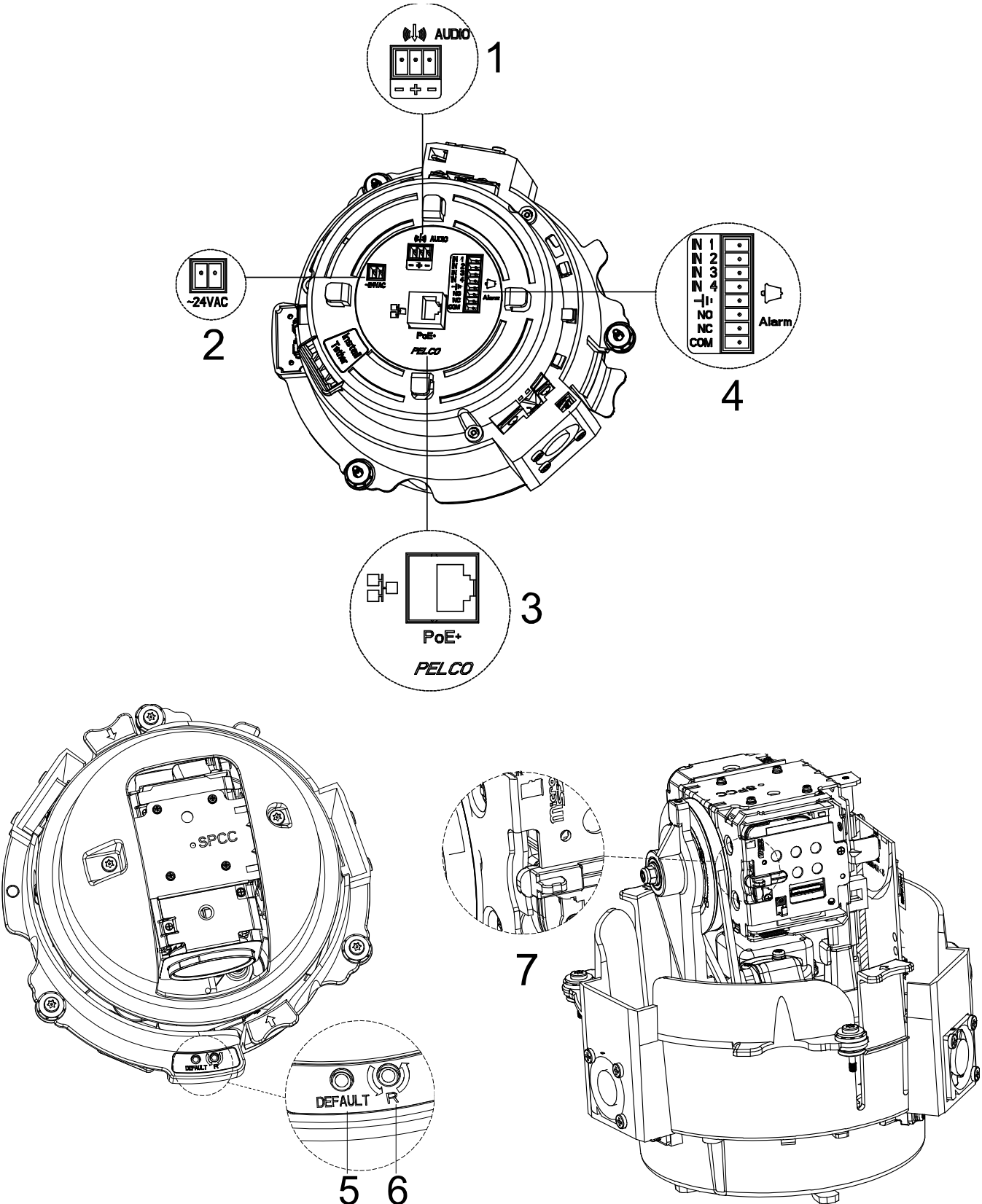
FIGURE 1-2: PICTORIAL INDEX
