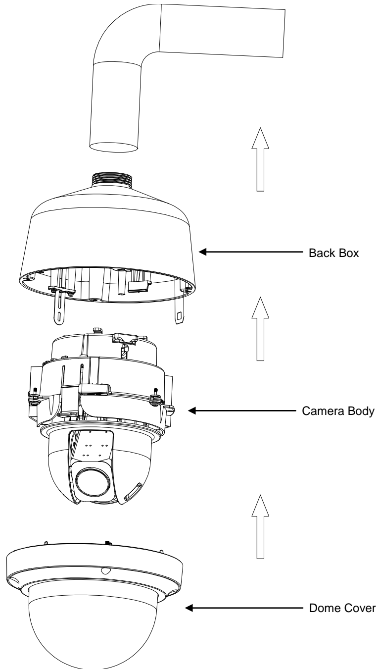
FIGURE 2-5: INDOOR / OUTDOOR PENDANT INSTALLATION
