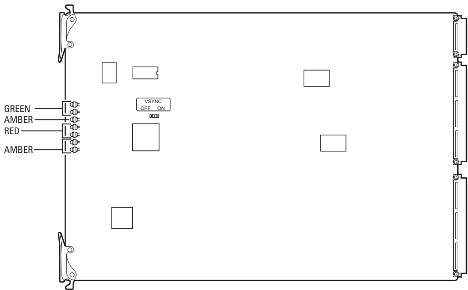
Figure 41. CM9780-VCC Card
