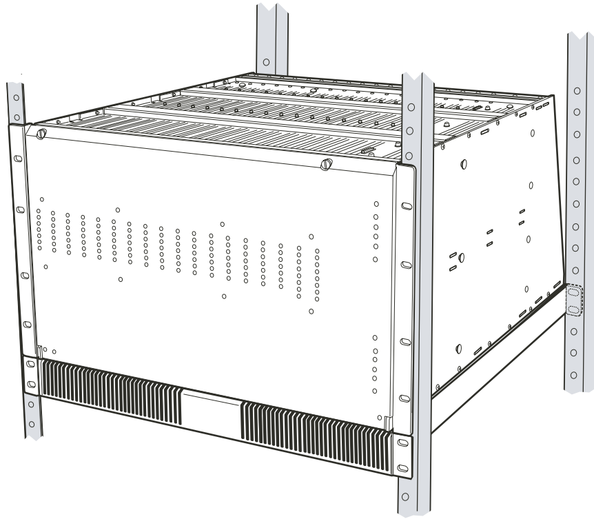
Figure 2. Mounting the CM9780-MXB on Top of the Mounting Baffle
