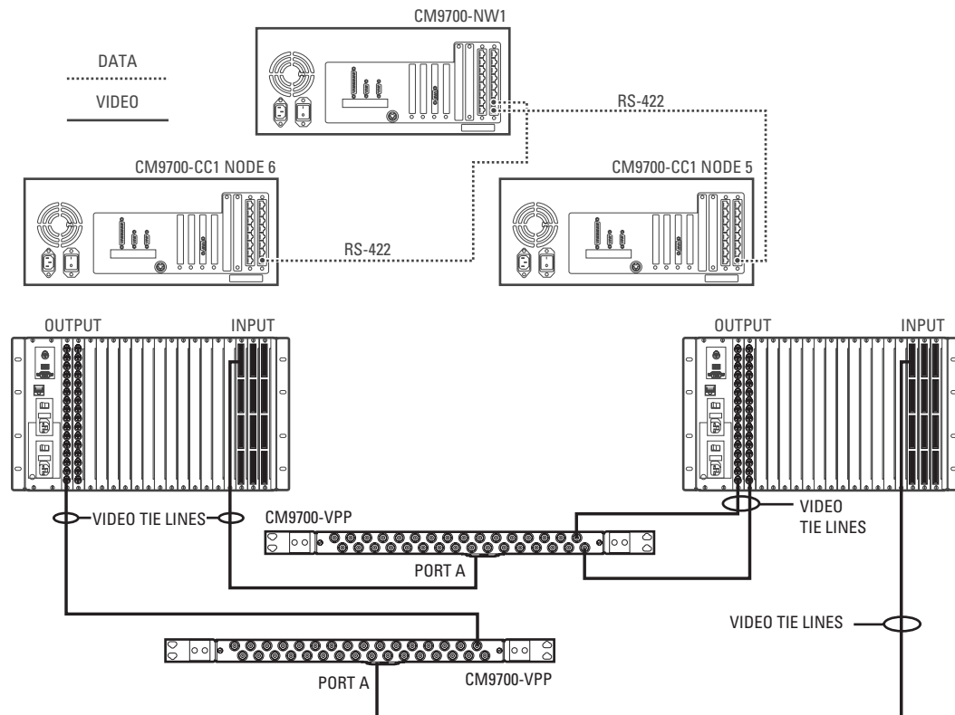
Figure 43. Sample Networked System
