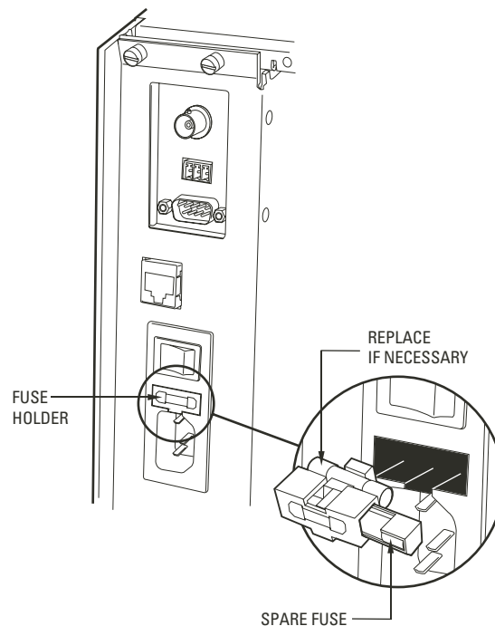
Figure 19. How to Replace a Power Supply Fuse
