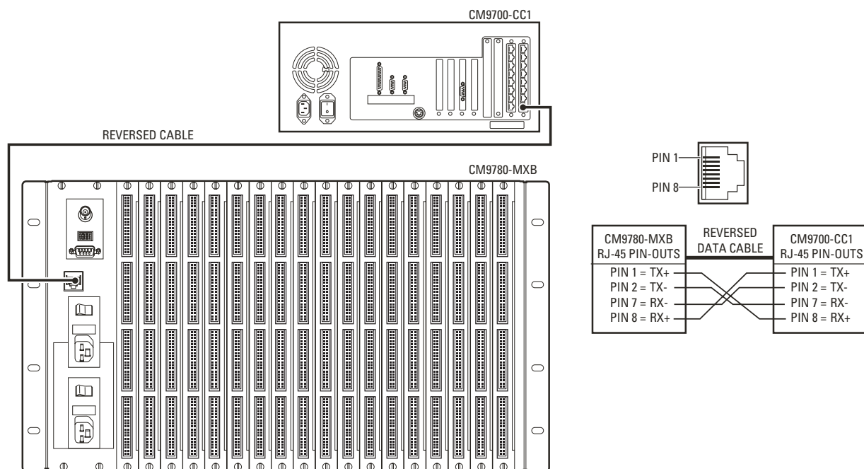
Figure 24. Sample CM9780-MXB to CM9700-CC1 Connection
