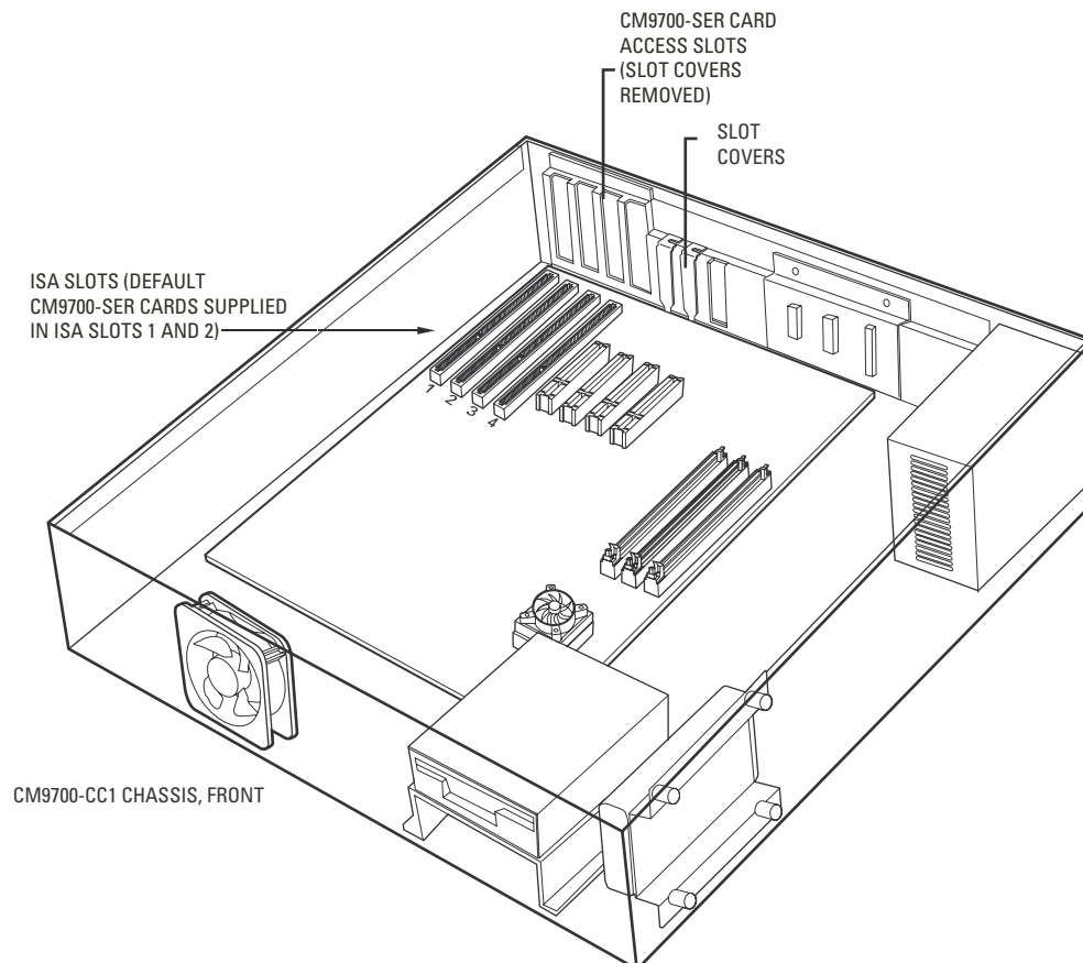
Figure 40. How to Install a CM9700-SER Card
