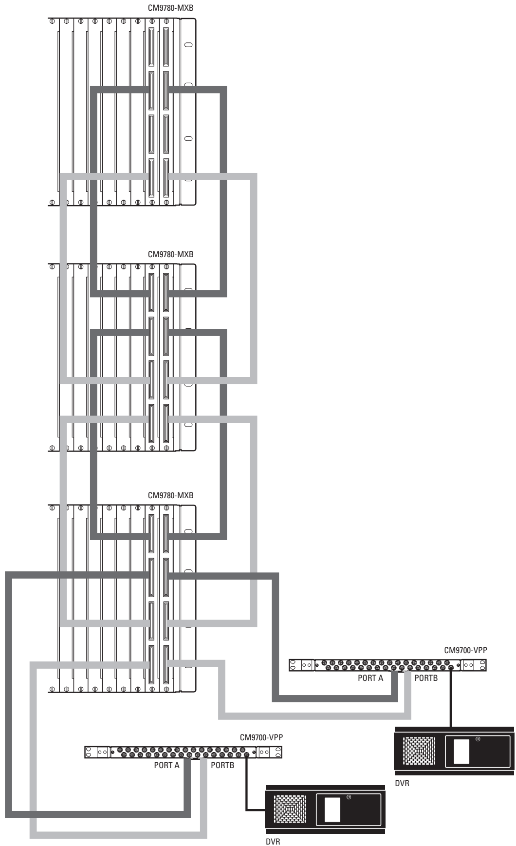
Figure 35. Looping Downframed Video with CM9700-VPP Patch Panels
