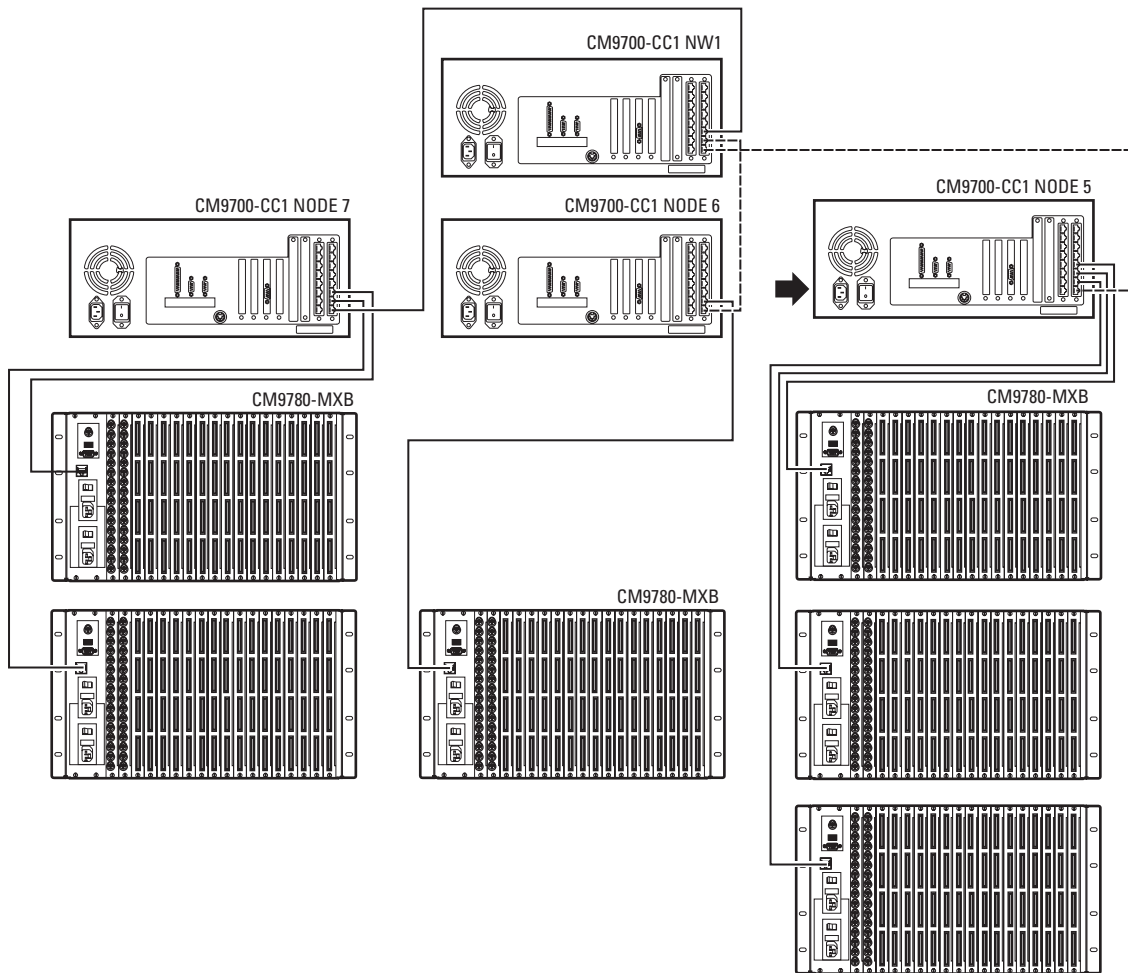
Figure 17. Sample Networked System
