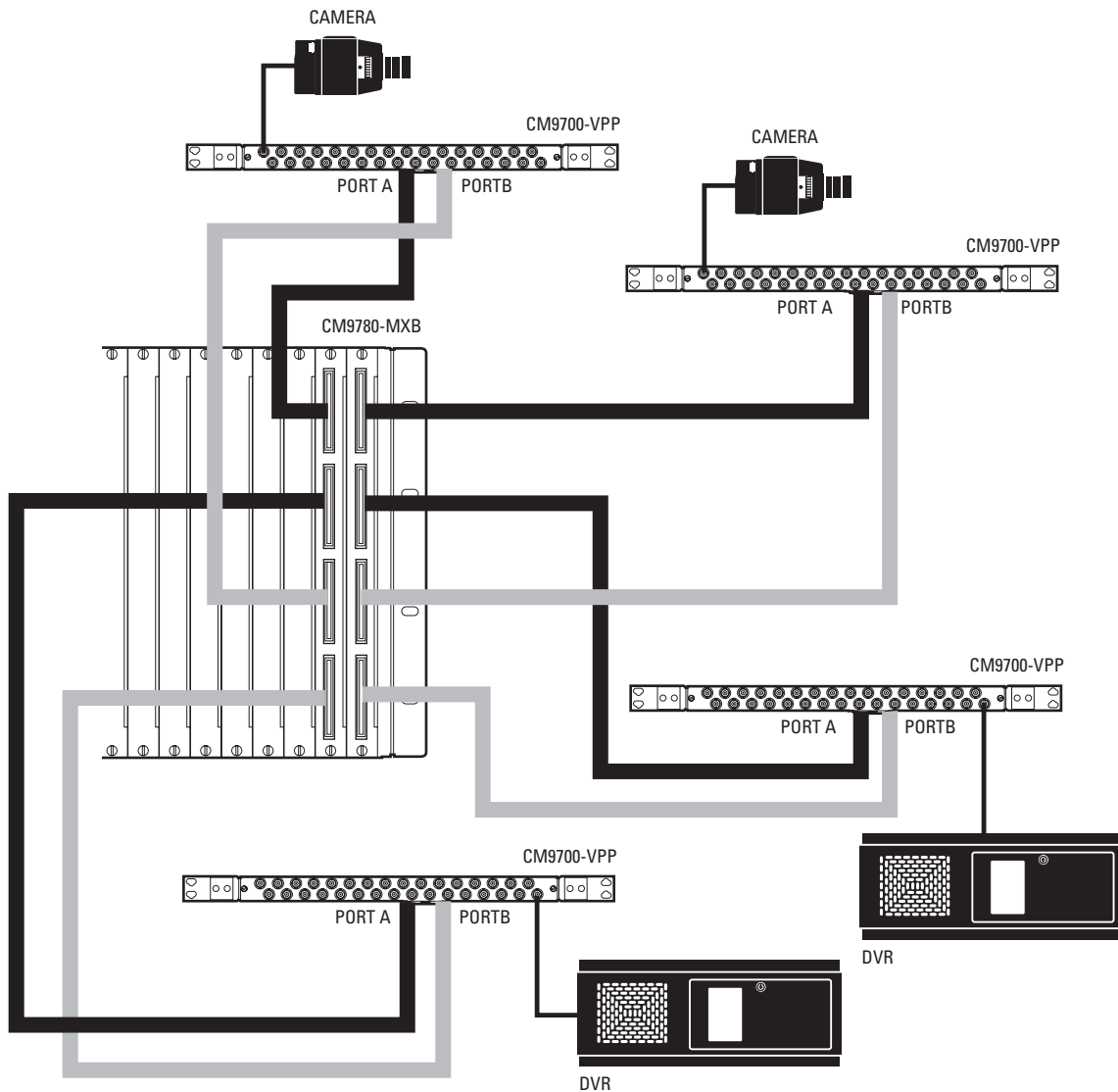
Figure 11. Looping Video Out from the CM9780-MXB
