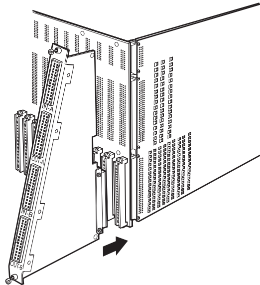
Figure 8. Insert a Rear Panel Video DFC Card (CM9780-DFC)
