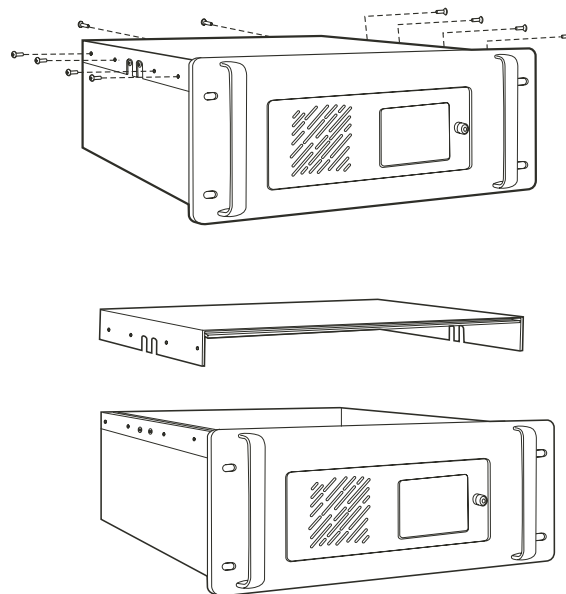
Figure 38. Removing the CC1 Top Cover
