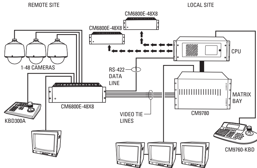
Figure 44. Sample Satellite System
