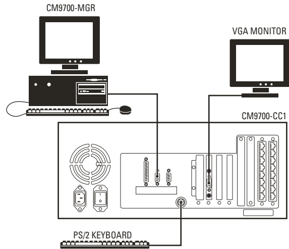
Figure 22. CM9700-CC1 Device Connections
