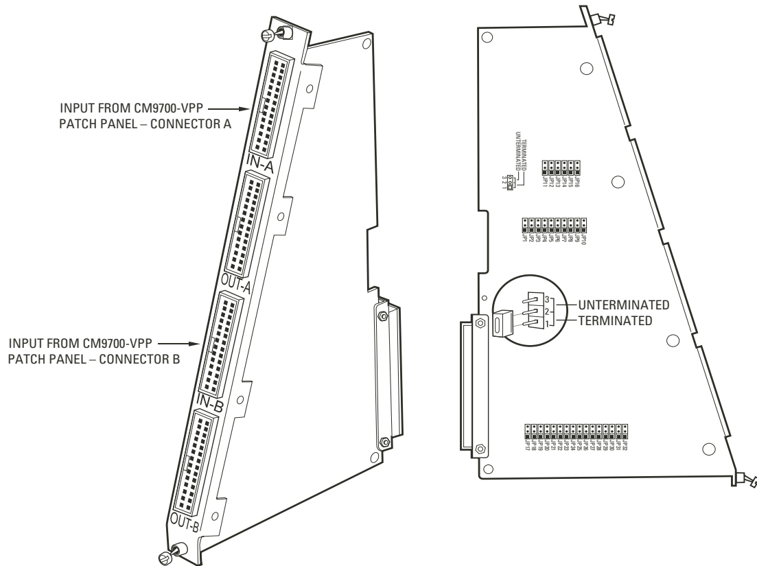
Figure 9. DFC Card
