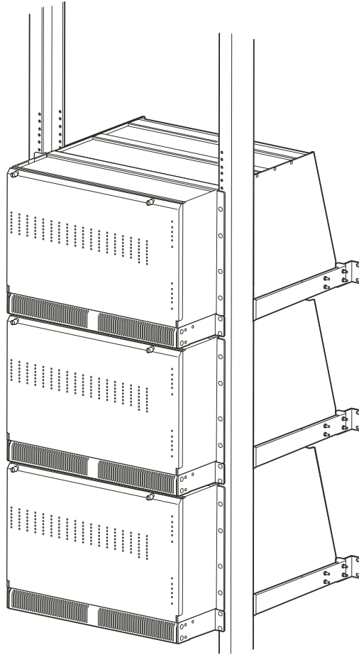
Figure 46. Mounting the CM9780-MXB in an Open Rack
