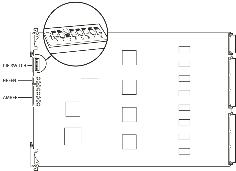
Figure 42. CM9780-VMC Card
