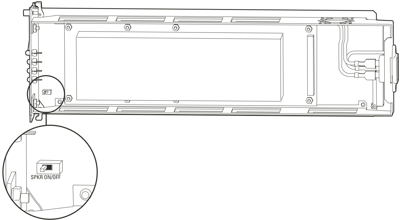
Figure 20. Power Supply Alarm Speaker Switch
