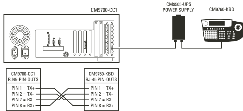
Figure 21. Connect the CM9760-KBD to the CM9700-CC1
