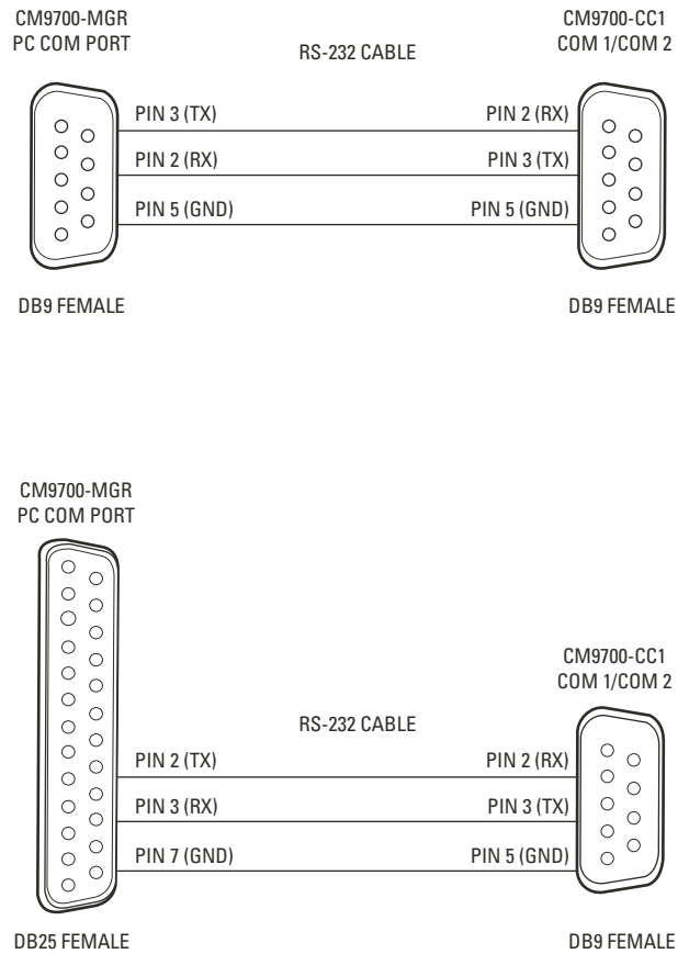
Figure 23. CM9700-MGR PC Pin-Out Detail
