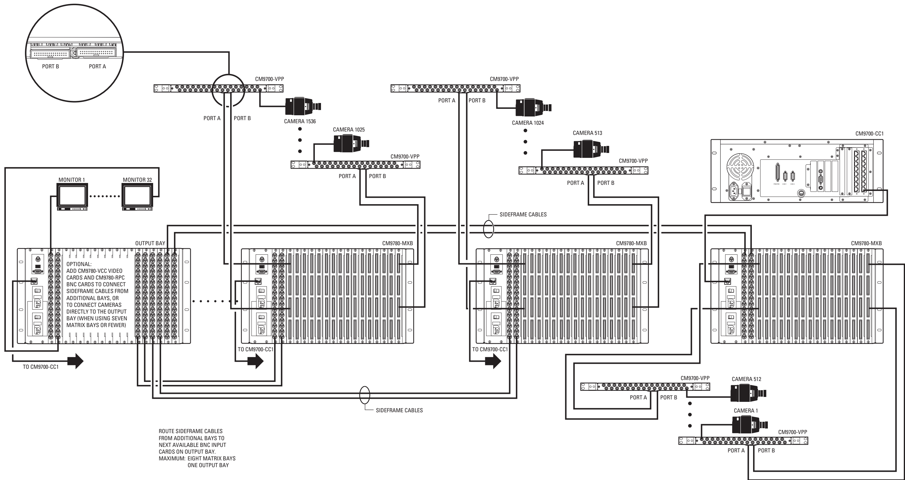
Figure 15. Sample Sideframing System Using CM9780-RPC Cards in the Output Bay (4098 Cameras Maximum)
