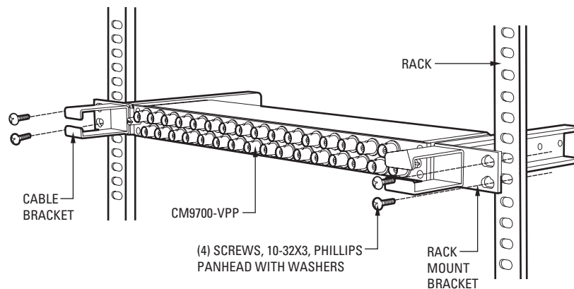
Figure 4. CM9700-VPP Horizontal Mount
