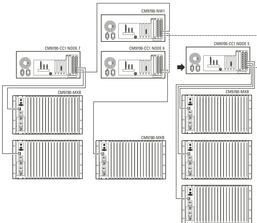
Figure 25. Sample CM9780-MXB and CM9700-CC1 Connections in a Networked System
