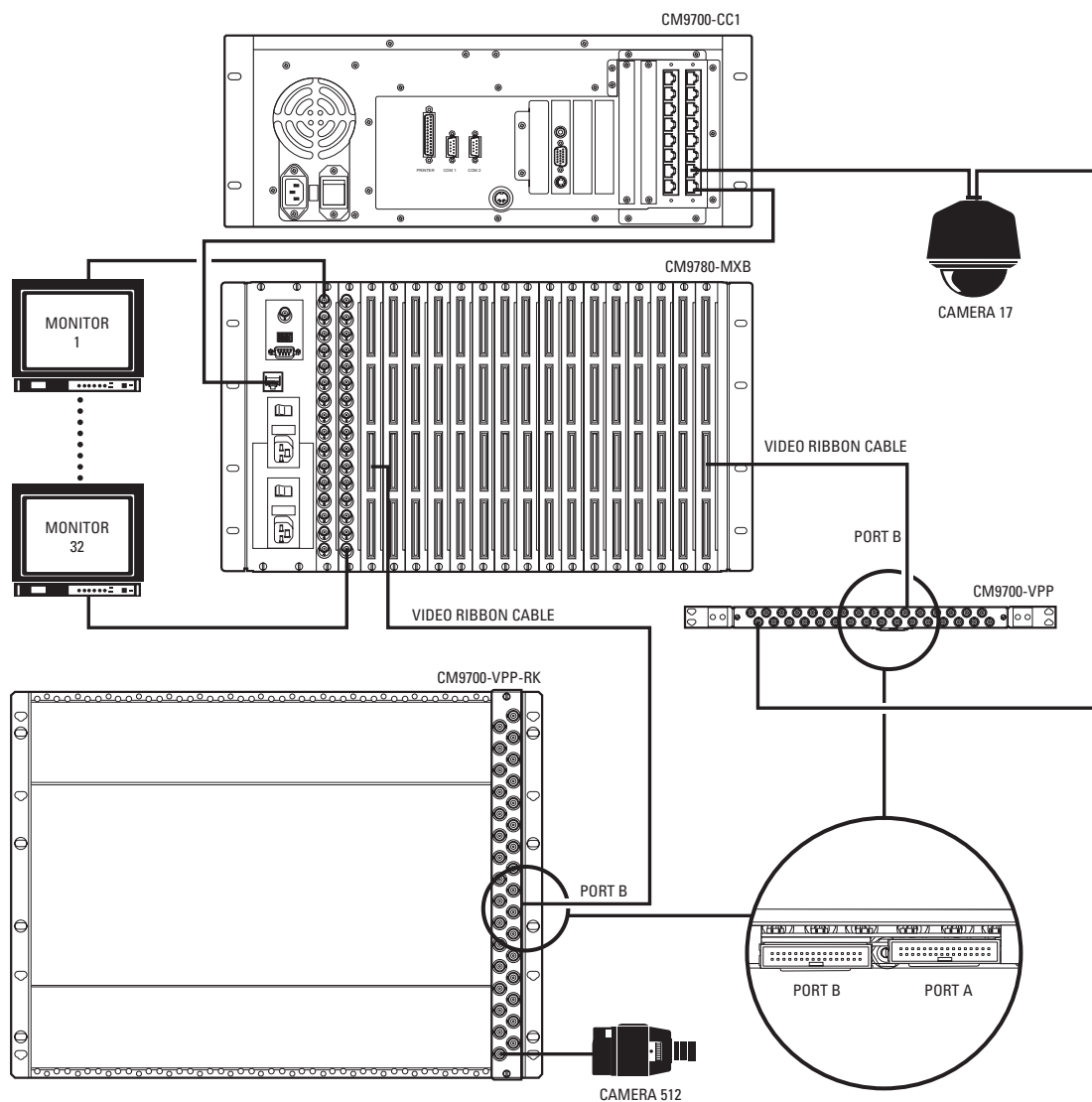
Figure 12. Sample CM9780 System with 512 Cameras and 32 Monitors
