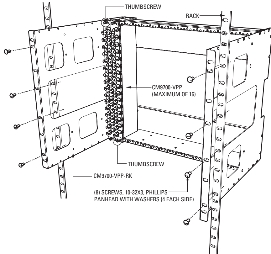
Figure 5. CM9700-VPP Vertical Mount
