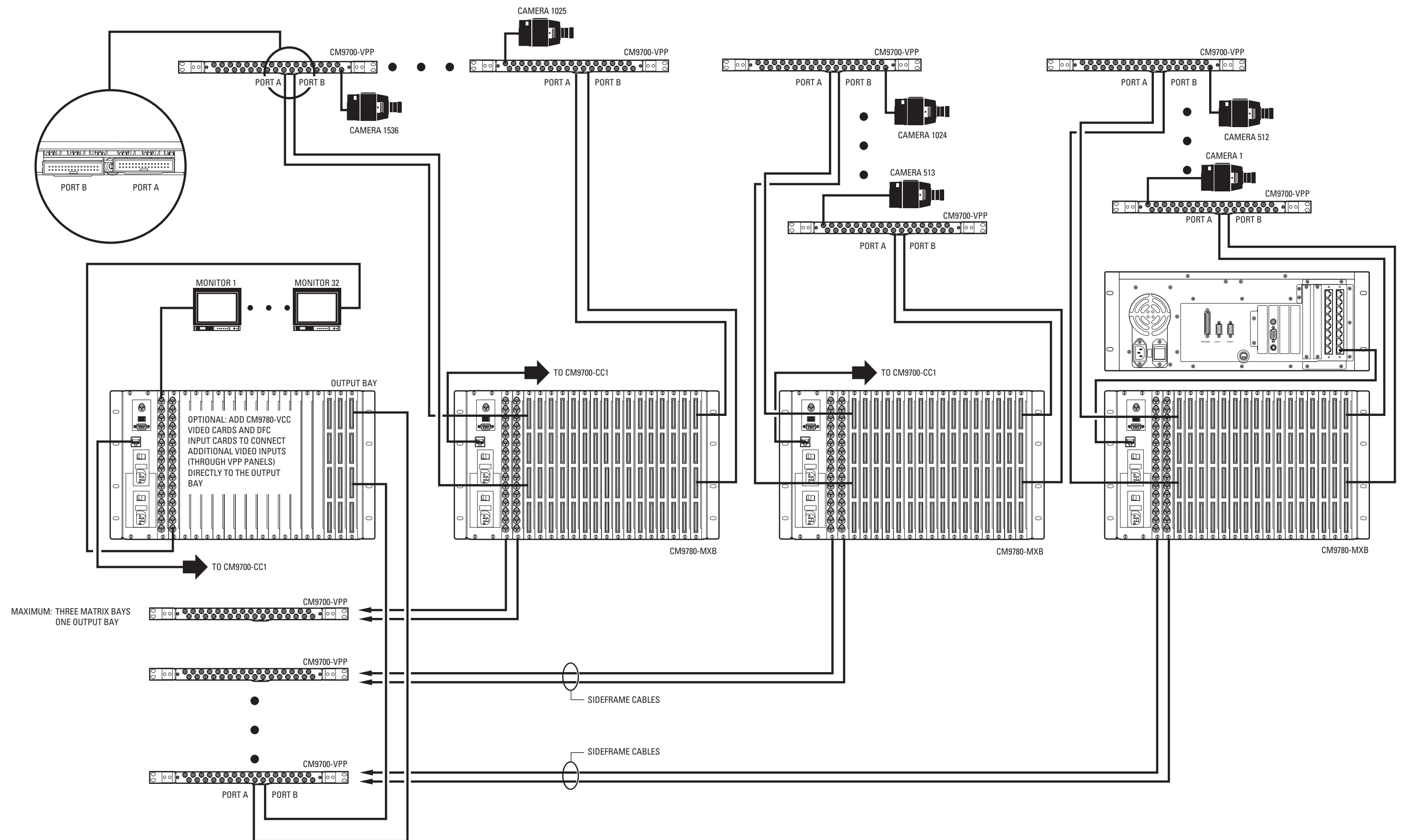
Figure 14. Sample Sideframing System Using CM9780-DFC Cards in the Output Bay (1952 Cameras Maximum)
