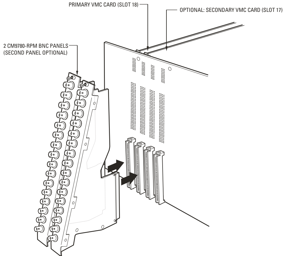
Figure 10. CM9780-MXB Matrix Bay—16 Monitor Output Connections for Each VMC Card
