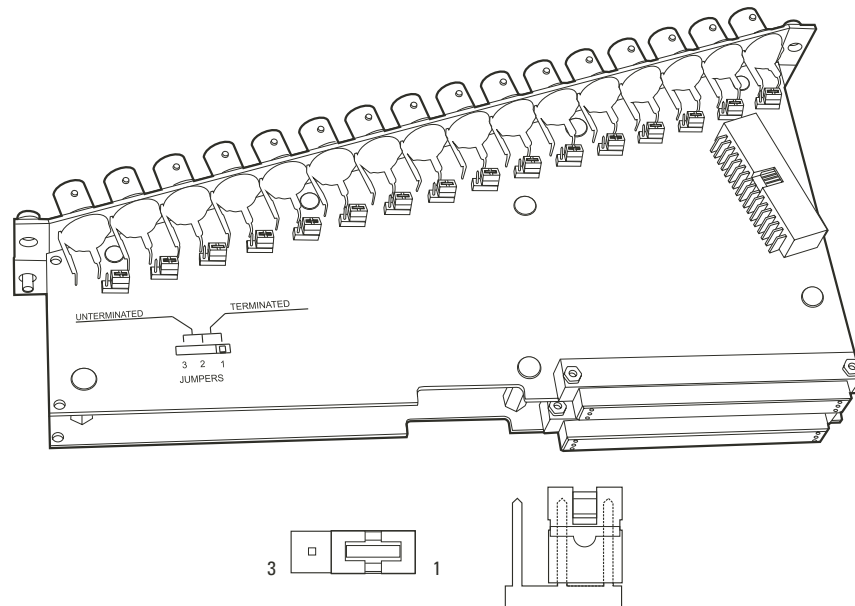
Figure 33. CM9780-RPC Termination Jumpers—Left Card
