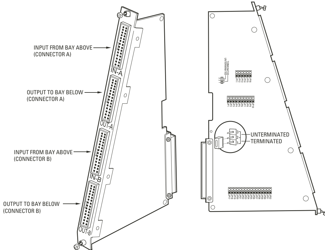
Figure 36. Downframing with the CM9780-DFC Card
