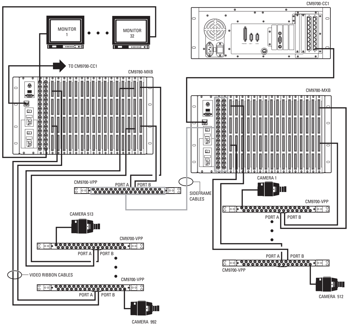
Figure 13. Sample System Using Sideframing from Bay to Bay
