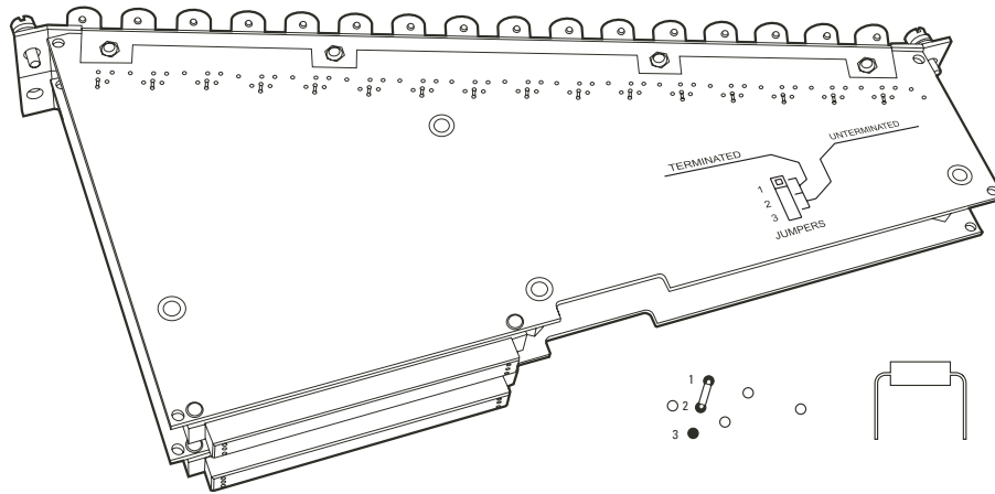
Figure 32. CM9780-RPC Termination Jumpers—Right Card
