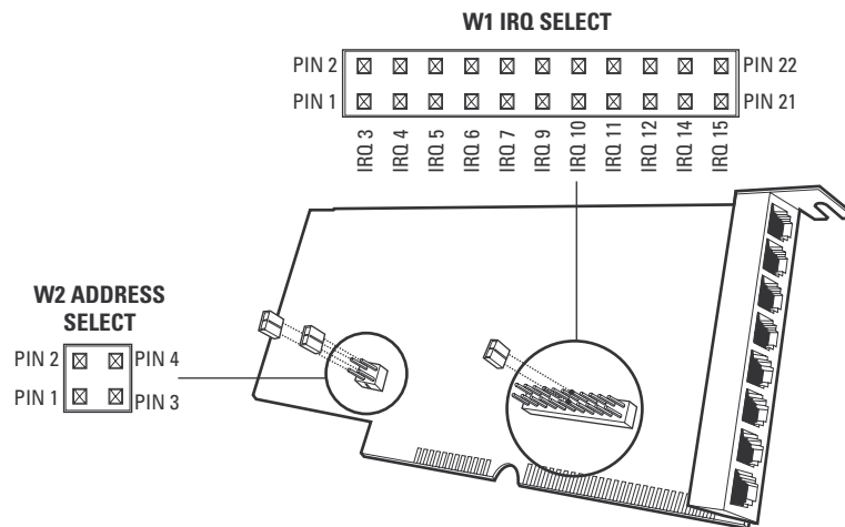
Figure 39. SER Card Jumper Assignments
