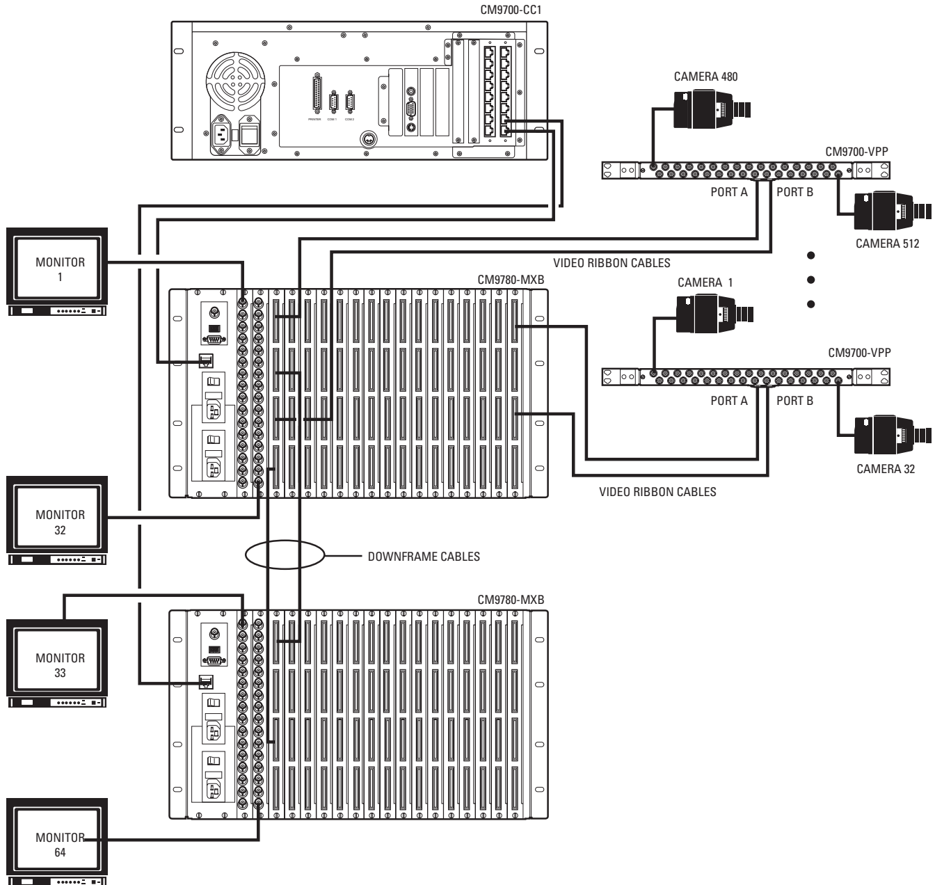
Figure 16. Sample Single-Node System with Downframing
