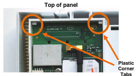
Figure 3: Module plastic corner tabs
