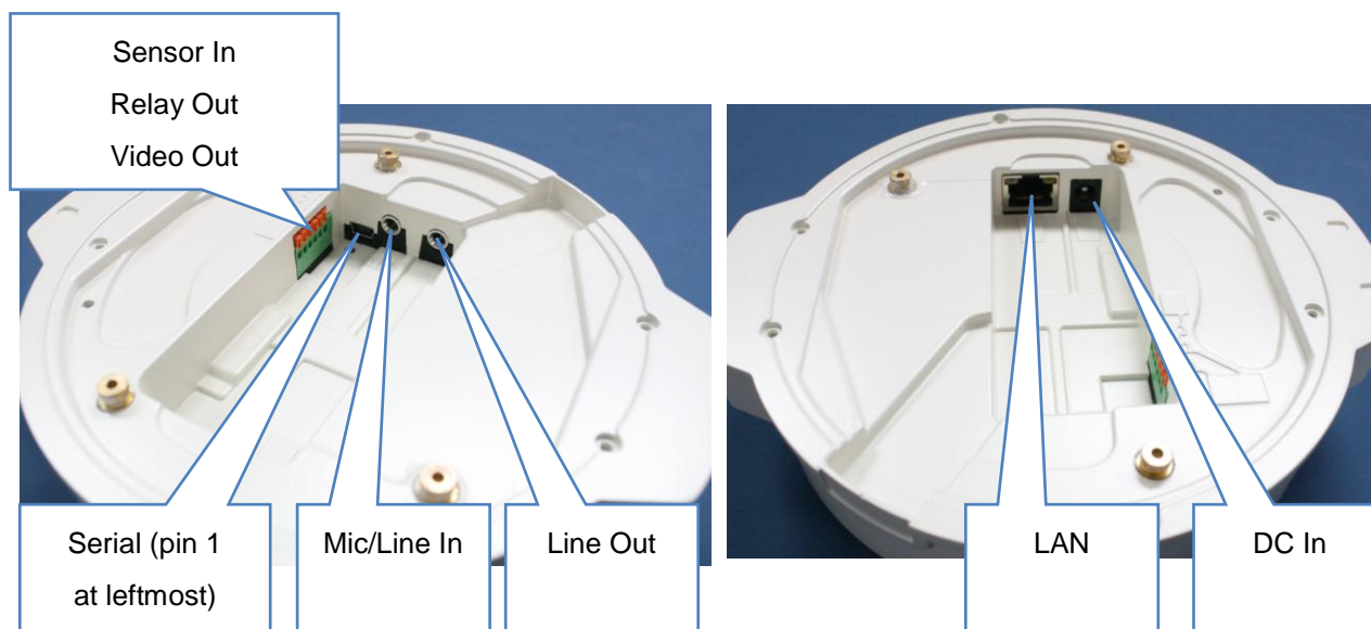
Figure 2-2. Rear panel of ONSIP O2DP7/O2IR24D7W
