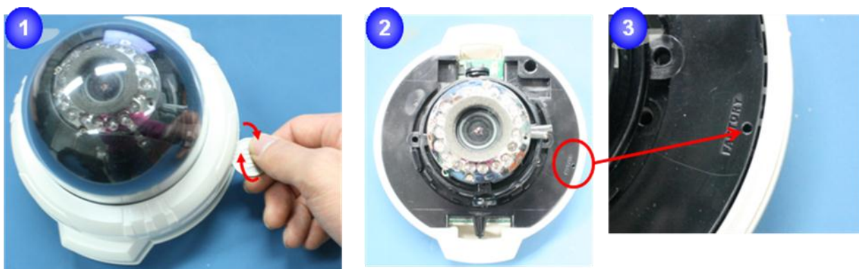
Figure 2-6 Factory Default switch of ONSIP O2DP7/O2IR24D7W
