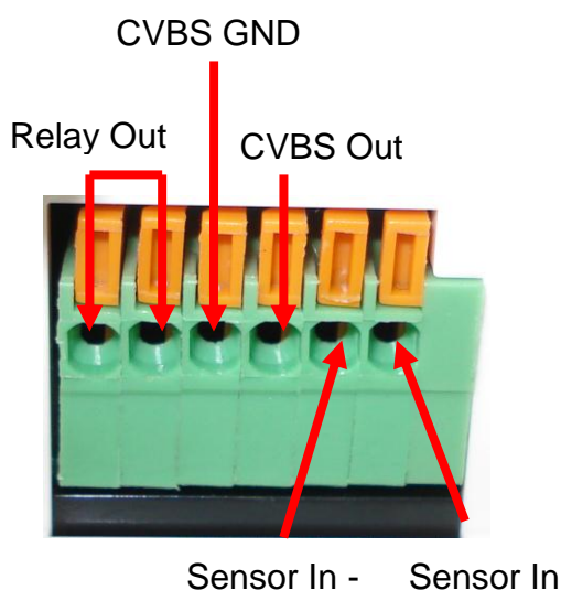
Figure 2-3 ALARM IN/OUT and Composite Video Output Terminal of ONSIP O2DP7/O2IR24D7W
