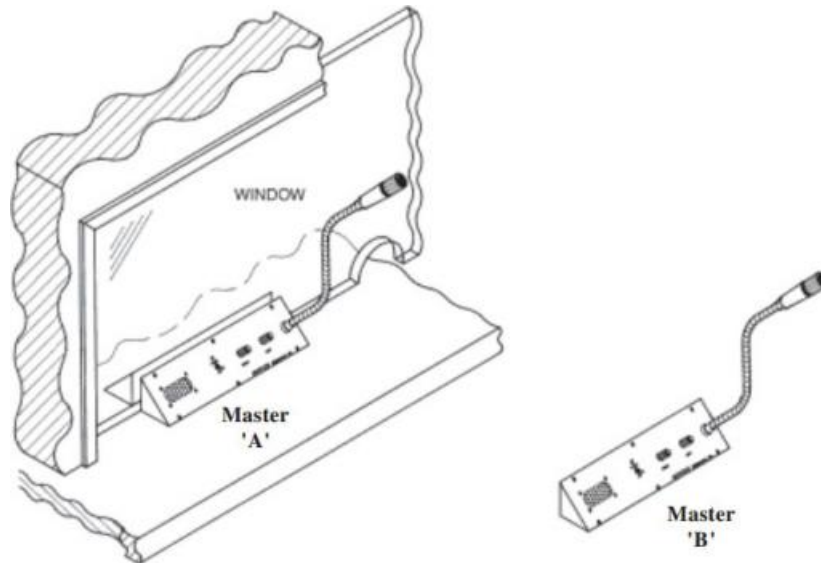
The Ideal Counter-Top Communication System Where It is Impractical to Cut a Hole In the Barrier
