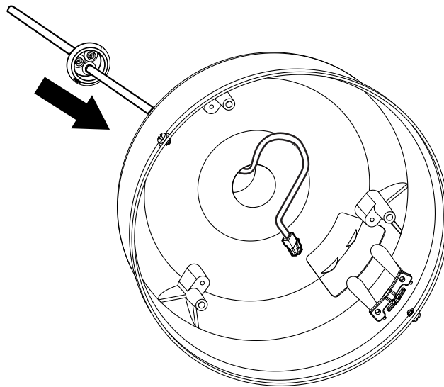
Figure 7. Pulling the Wiring into the Back Box
