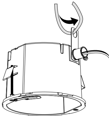
Figure 2. Safety Chain
