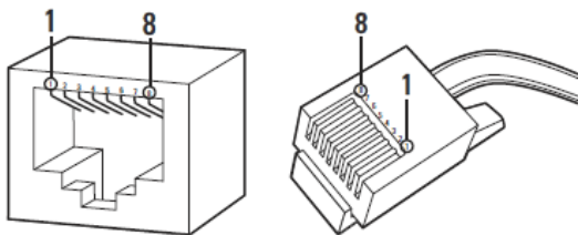
Figure 19. Pin Numbering
