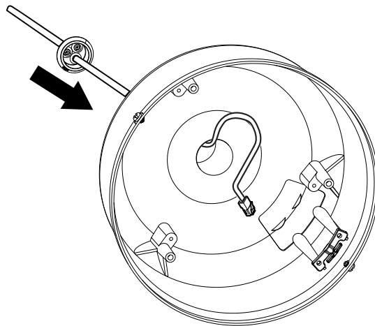
Figure 10. Dome Drive with Grommet Installed on Back
