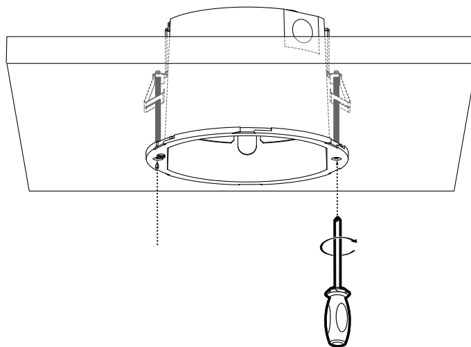
Figure 3. Installing the Back Box: In-Ceiling Models
